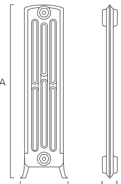
footed end section depth = 174mm
